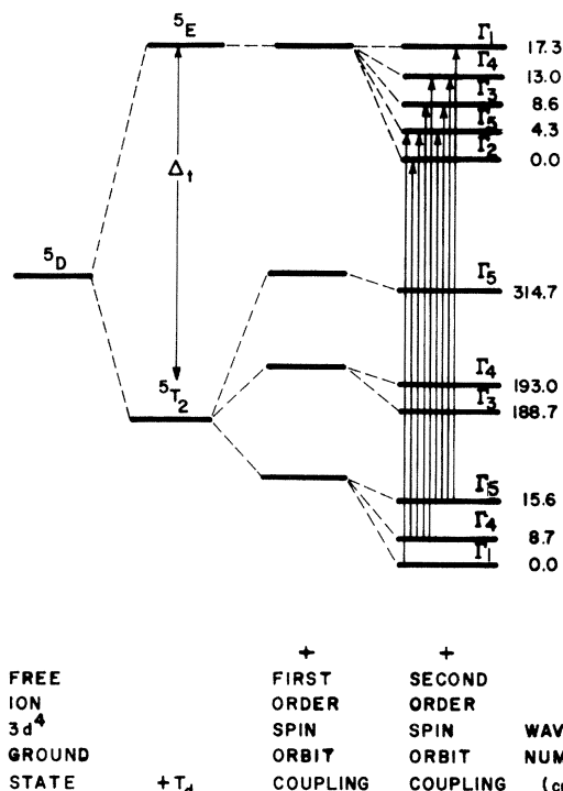
FIG. 5. Energy levels of tetrahedrally coordinated \text{Cr}^{+2} ( 3d^4 ) as predicted by crystal field theory. Allowed electric dipole transitions and wave numbers of energy levels are shown.
